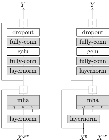
Figure 5.6: Self-attention block (left) and cross-attention block (right).
